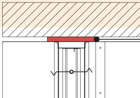
FIRESTOP CAULK INSTALLED THROUGHOUT ANNULAR SPACE
