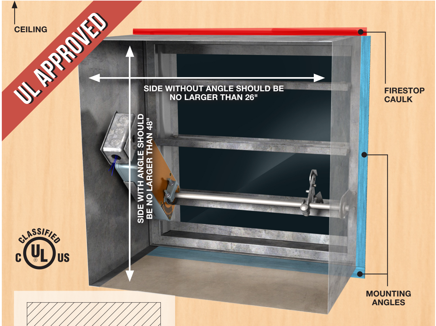
FIRESTOP CAULK INSTALLED THROUGHOUT ANNULAR SPACE
